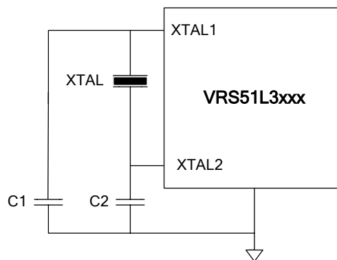
FIGURE 51: VRS51L3xxx EXTERNAL CRYSTAL OSCILLATOR CONFIGURATION
