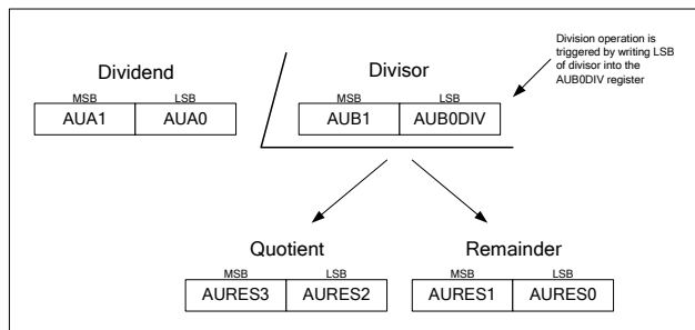
FIGURE 43: ARITHMETIC UNIT DIVISION OVERVIEW
