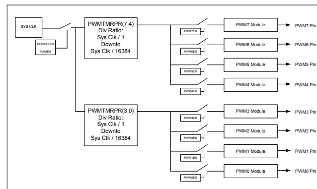
FIGURE 40: PWM AS TIMERS OVERVIEW
