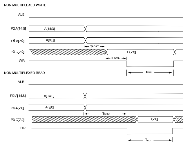
FIGURE 8: NON-MULTIPLEXED EXTERNAL DATA MEMORY ACCESS
