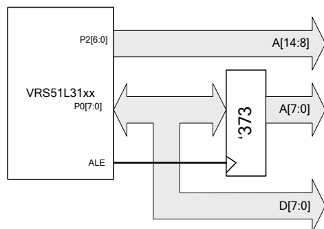
FIGURE 10: MULTIPLEXED EXTERNAL DATA MEMORY ACCESS REPRESENTATION
