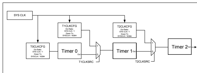
FIGURE 20: TIMER CHAINING
