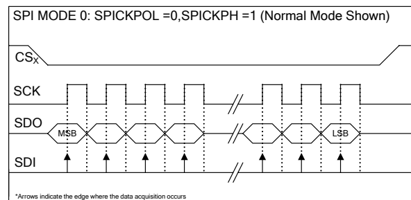
FIGURE 24: SPI MODE 0
