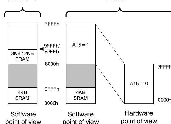
FIGURE 9: EXTBUSEN AND FRAMEN BIT CONFIGURATION EXTBUSEN = 1 FRAMEN = 1
