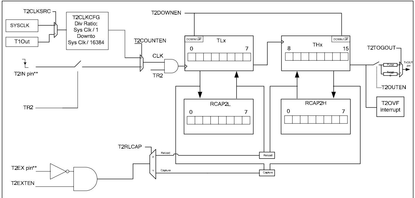
FIGURE 19: TIMER 2 FUNCTIONAL DIAGRAM
