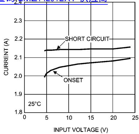
Current Limit 1.8V_{OUT} @ 25^{\circ}C 查询"LMZ14201EXT"供应商
