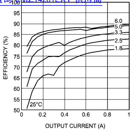
Efficiency 24V Input @ 25°C 查询LMZ14201EXT"供应商"
