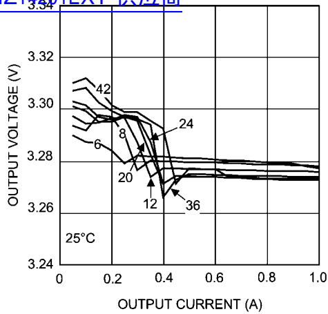
Line and Load Regulation @ 25°C 查询"LMZ14201EXT"供应商
