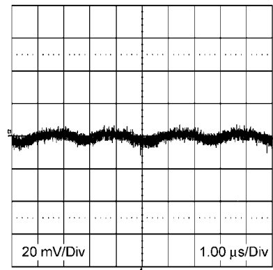
Output Ripple 24V_{IN} 3.3V_O 1A, BW = 200 MHz
