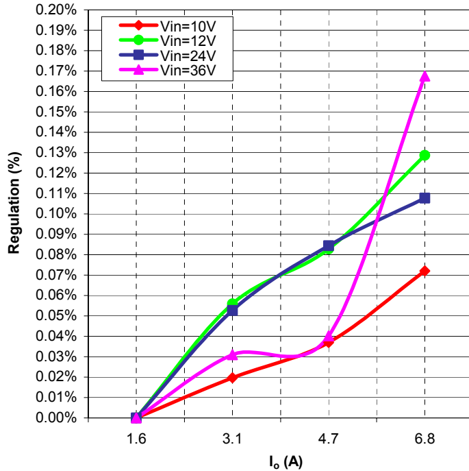
Graph 5: LV12S24-150 Load Regulation ( \pm RS Pins Open)
