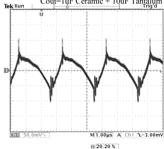
Photo 11: Output Voltage Ripple (Spike) V_{in}=24V , I_{out} = 6.25A C_{out}=1\mu F Ceramic + 10\mu F Tantalum
