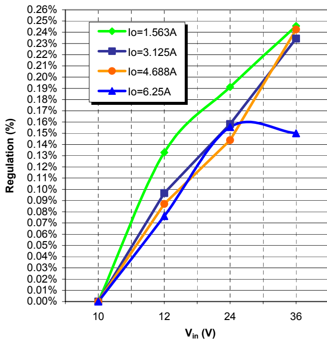
Graph 7: LV12S26-150 Line Regulation ( \pm RS Pins Open)
