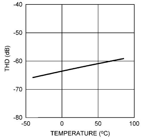
THD vs. TEMPERATURE (ADC10D1500)
