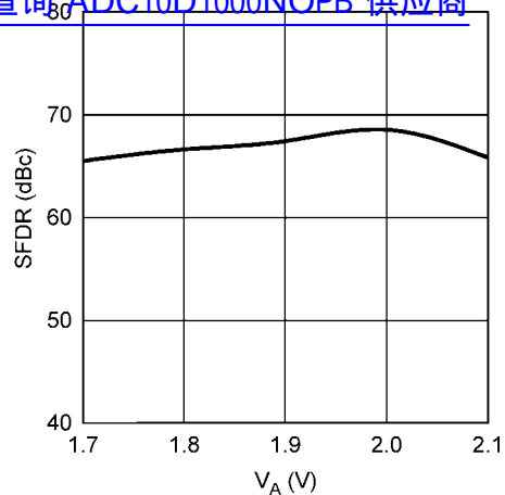
SFDR vs. SUPPLY VOLTAGE (ADC10D1000) 查询"ADC10D1000NOPB"供应商
