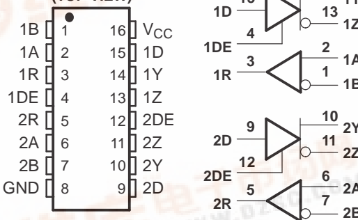
SN65LVDS051 D OR PW PACKAGE (TOP VIEW)
