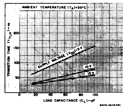
Fig.9 - Typical low-to-high transition time vs. load capacitance.
