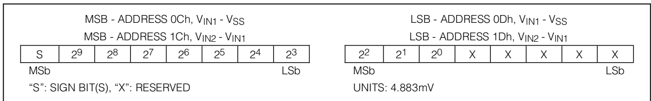
Figure 4. Voltage Register Format
