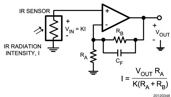
FIGURE 17. IR Radiation Sensor
