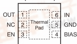
TPS720xx DRV PACKAGE 2mm x 2mm SON-6 (TOP VIEW)
