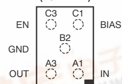
TPS720xx YZU PACKAGE 1,33mm x 0,96mm WCSP-5 (TOP VIEW)
