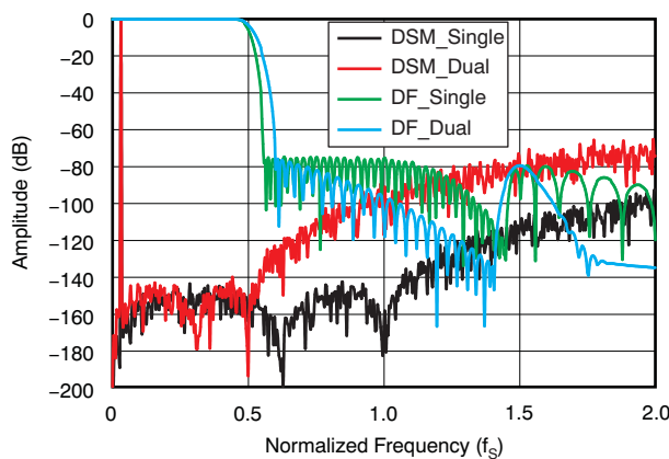
Figure 31. ADC \Delta\Sigma Modulator and Digital Filter Characteristic
