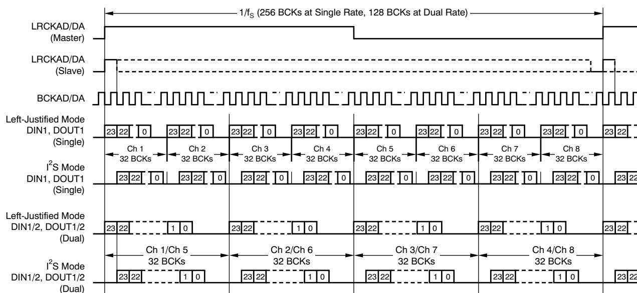
Figure 40. Audio Data Format: 24-Bit TDM Format (SCKI = 128 f s , 256 f s , and 512 f s Only)
