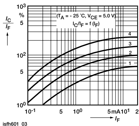
Fig. 3 - Current Transfer Ratio vs. Diode Current
