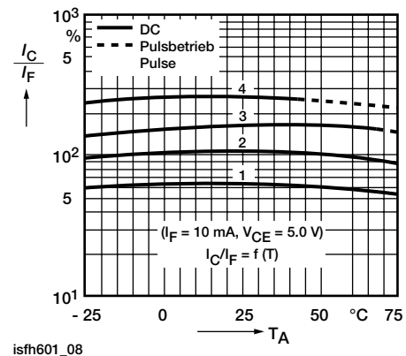
Fig. 8 - Current Transfer Ratio vs. Diode Current
