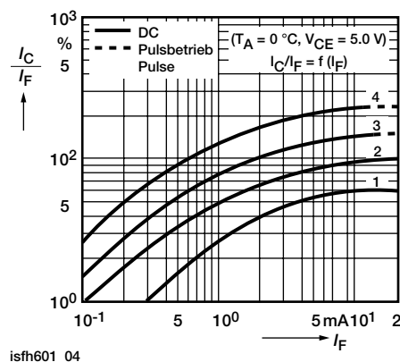
Fig. 4 - Current Transfer Ratio vs. Diode Current
