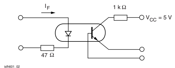
Fig. 2 - Switching Operation (With Saturation)
