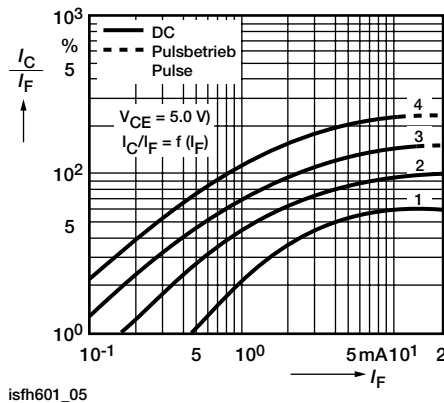
Fig. 5 - Current Transfer Ratio vs. Diode Current
