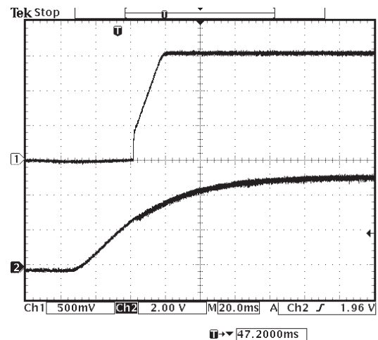
Figure 11: Typical Power-up Characteristic (Channel 1: V_o , Channel 2: V_{in} )
