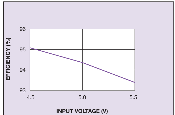
Figure 9: Efficiency vs Line ( V_o = 3.3\text{ V} )
