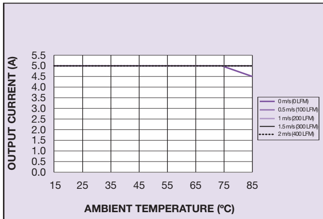
Figure 8: Derating Curve ( V_o = 3.3\text{ V} )
