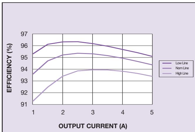
Figure 10: Efficiency vs Load ( V_o = 3.3\text{ V} )
