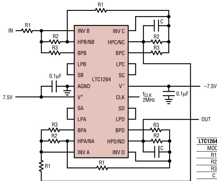
100kHz, 8th Order Notch Filter, f_{CLK}/f_{CENTER} = 20:1
