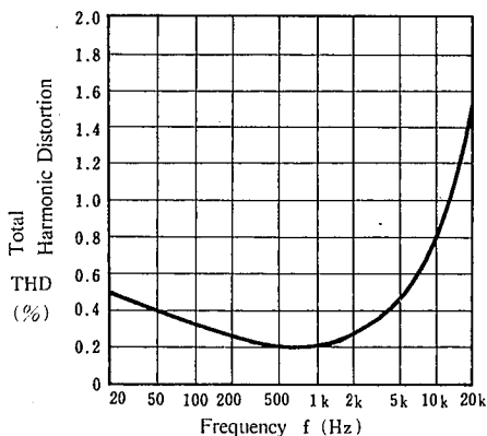
Total Harmonic Distortion vs. Frequency (V + = 6V, R L = 8Ω, P 0 = 125mW, A v = 26dB, T_a = 25^\circ\text{C} )
