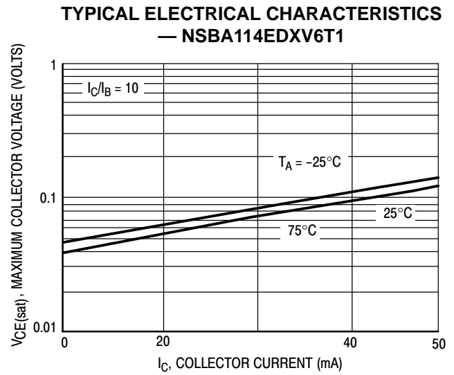
Figure 2. V CE(sat) versus I C
