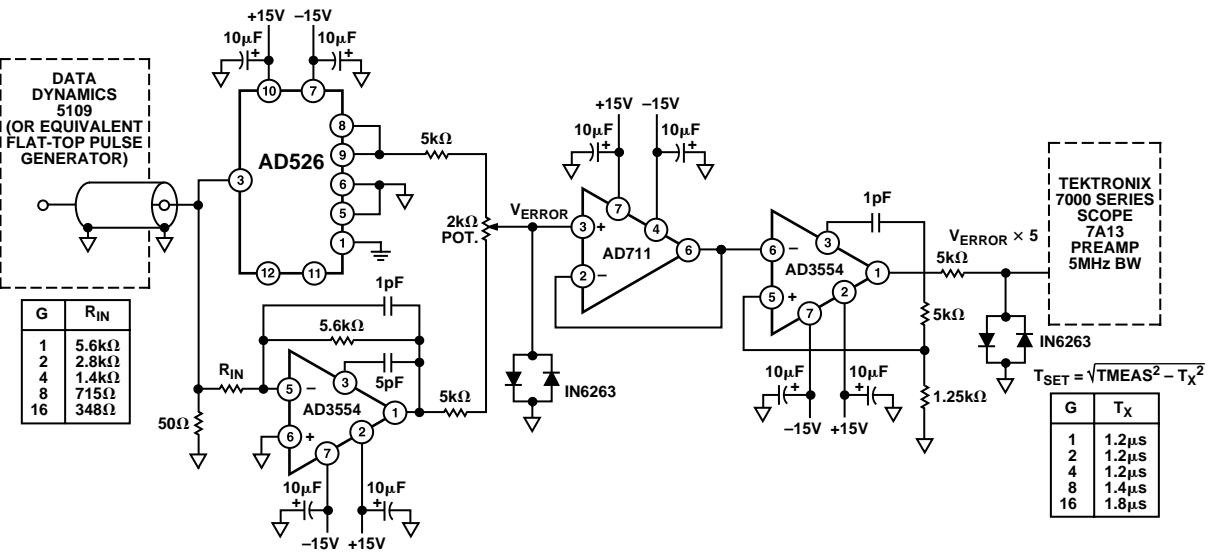
Figure 31. Settling Time Test Circuit
