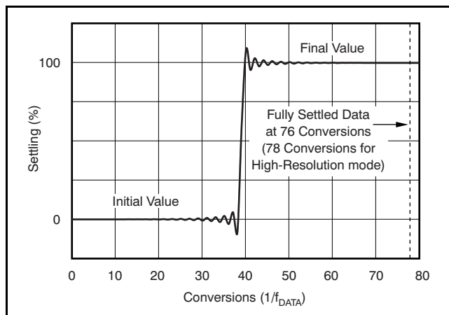
Figure 62. Step Response
