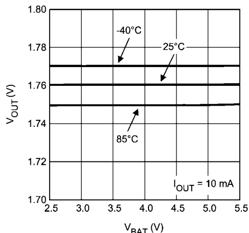
LDO Output Voltage vs. Supply Voltage
