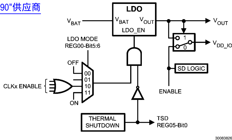
FIGURE 11. Linear Regulator Block Diagram
