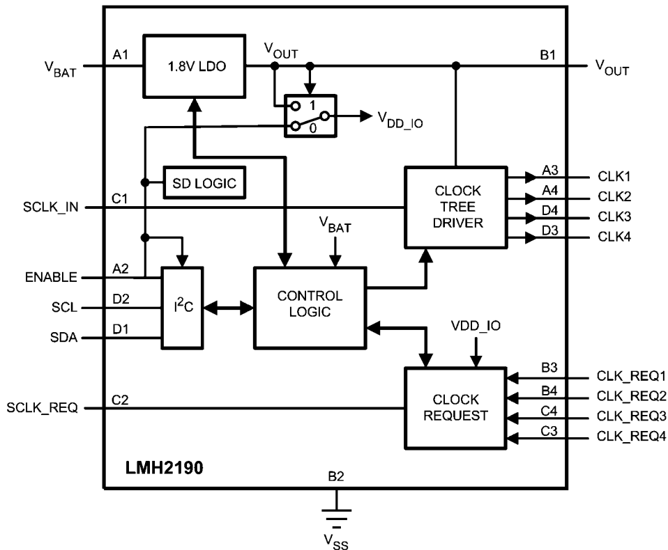
LMH2190
