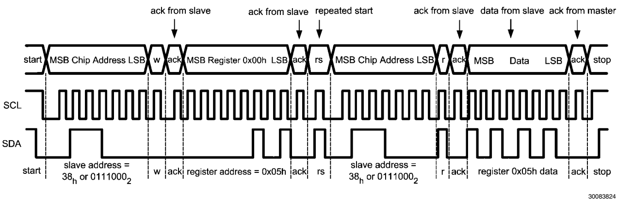
FIGURE 16. Example I 2 C Read Cycle
