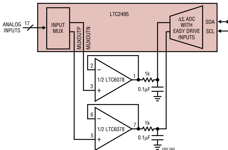
External Buffers Provide High Impedance Inputs and Amplifier Offsets are Automatically Cancelled
