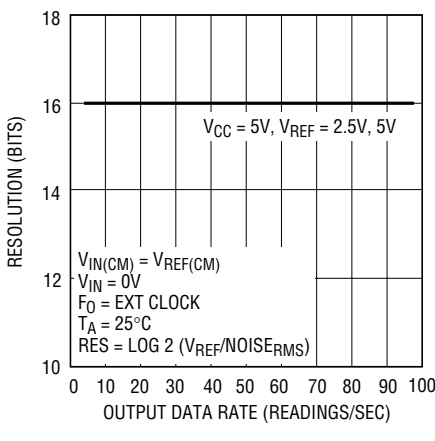
Figure 36. Resolution ( Noise_{RMS} \leq 1LSB ) vs Output Data Rate and Temperature
