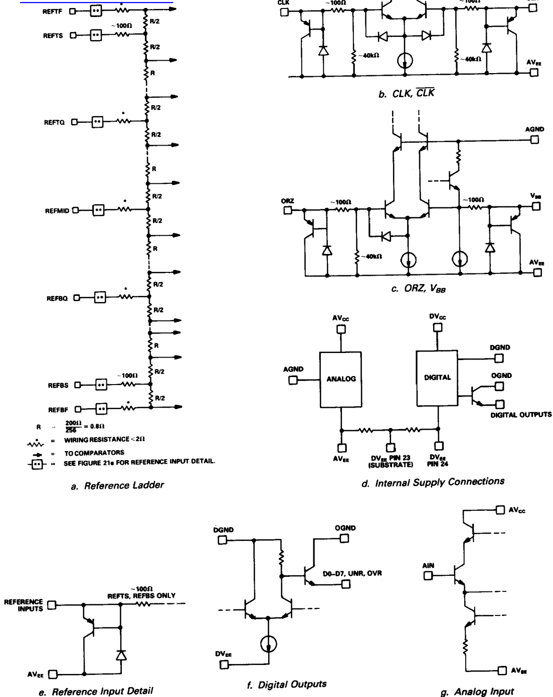
Figure 21. Equivalent Circuits
