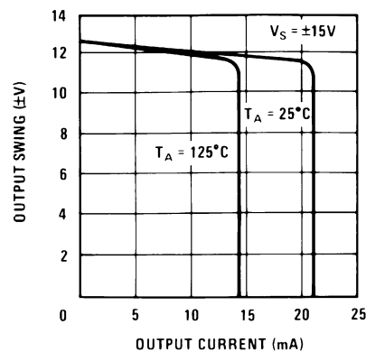
Current Limiting
