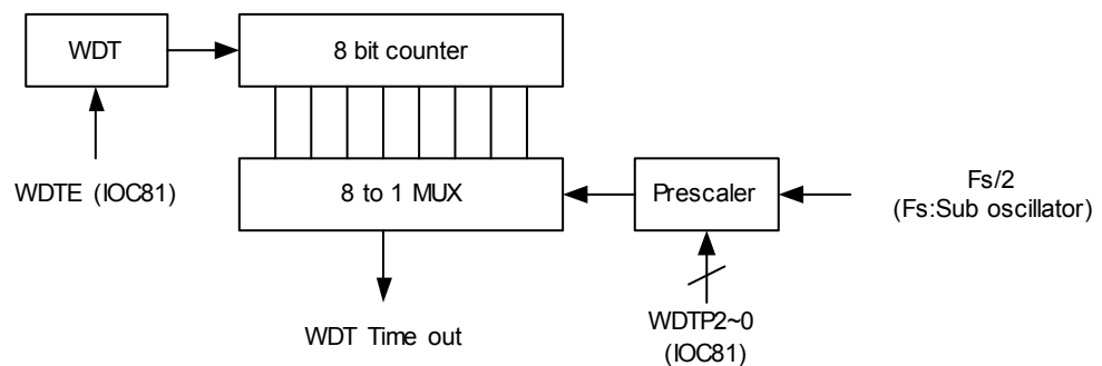
Fig. 7(b) Block Diagram of WDT
