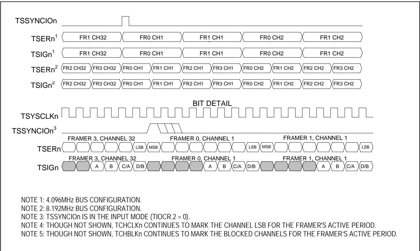
Figure 11-26. E1 Transmit-Side Interleave Bus Operation—BYTE Mode
