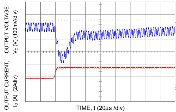
Figure 15. Transient Response to Dynamic Load Change from 50% to 100% at 28Vin, C_{ext} = 3 \times 10\mu F ceramic, C_{Tune} = 470pF & R_{Tune} = 150\Omega
