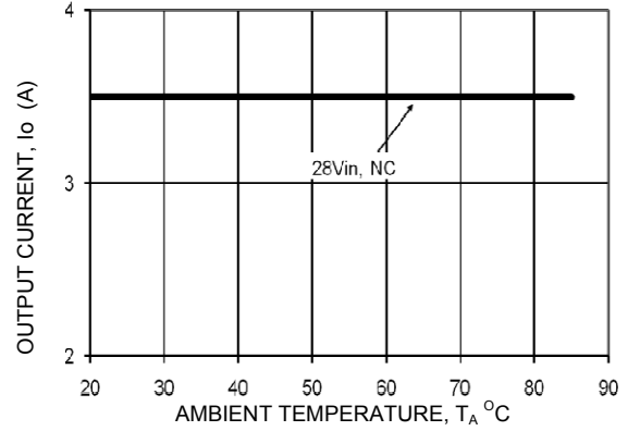
Figure 13. Derating Output Current versus Ambient Temperature and Airflow.
