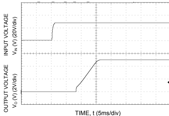
Figure 11. Typical Start-up Using Input Voltage ( V_{IN} = 28V , I_o = I_{o,max} ).
