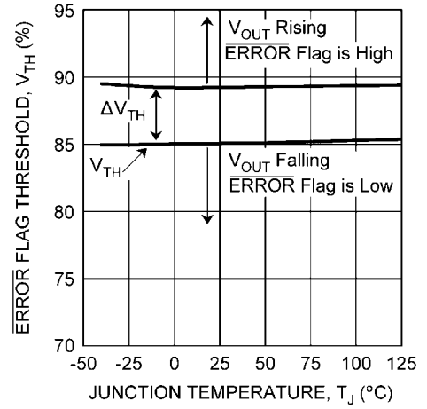
V OUT ERROR Flag Threshold vs Temperature
