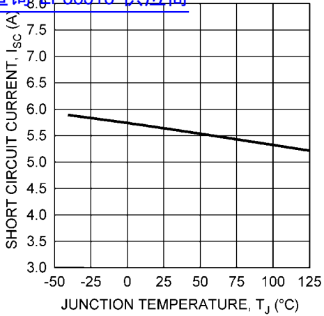
Current Limit vs Temperature 查询"LP38513"供应商
