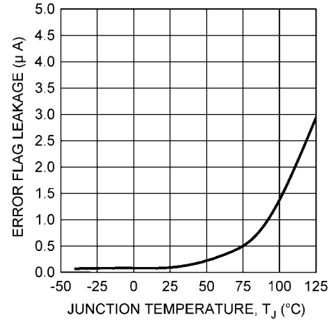
ERROR Flag Leakage vs Temperature
