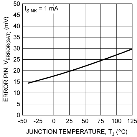
ERROR Flag Low vs Temperature
