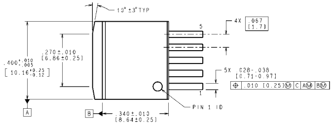
TO220 5-lead, Molded, Stagger Bend Package NS Package Number T05D
