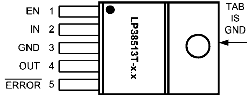
Top View TO-220 5 Pin Package
