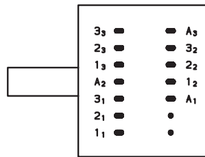
3 POLES 2 - 3 POSITIONS
