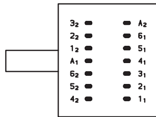
2 POLES 2 - 6 POSITIONS
