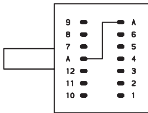
1 POLE 2 - 12 POSITIONS
