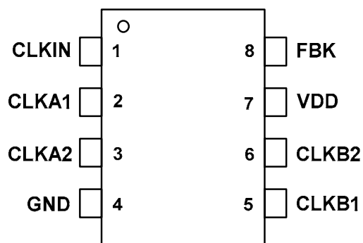
8-Pin SOIC
