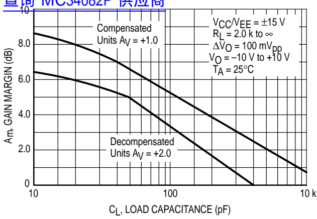
Figure 20. Gain Margin versus Load Capacitance
