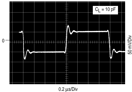
Figure 26. Small Signal
