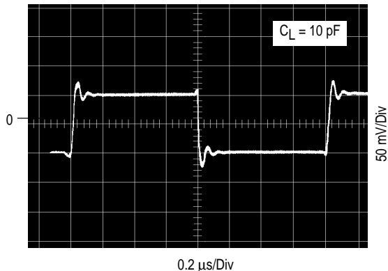
Figure 24. Small Signal
