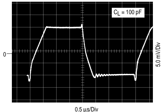
Figure 25. Large Signal
