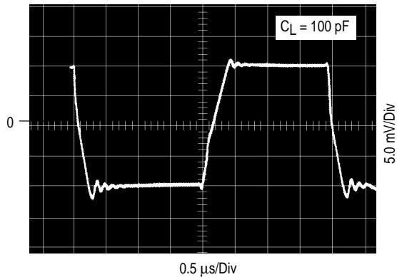
Figure 27. Large Signal
