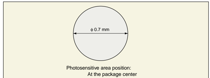
■ Figure 5 CXA2701GA Acceptance Pattern Dimensions
