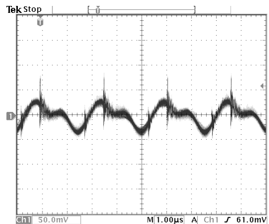
Photo 9: Output Voltage Ripple (20 MHz BW) Vin=24V, Iout=1.25A Cout=1uF Ceramic + 10uF Tantalum
