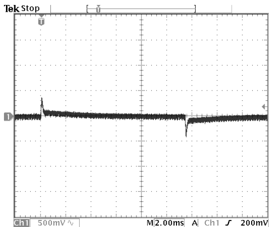
Photo 7: Transient Response 50% to 100% Vin=24V, Iout = 6.25 to 12.5A Cout=1uF Ceramic + 10uF Tantalum
