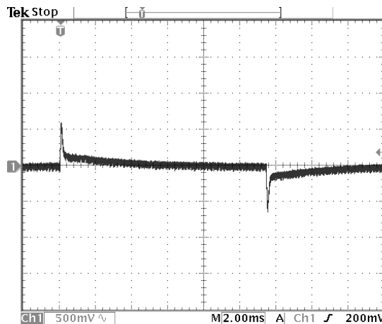
Photo 8: Transient Response Min Load to Max Load Vin=24V, Iout = 1.25 to 12.5A Cout=1uF Ceramic + 10uF Tantalum
