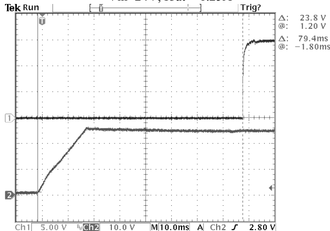
Photo 1: Remote Turn On Vin=24V, Iout = 1.25A
