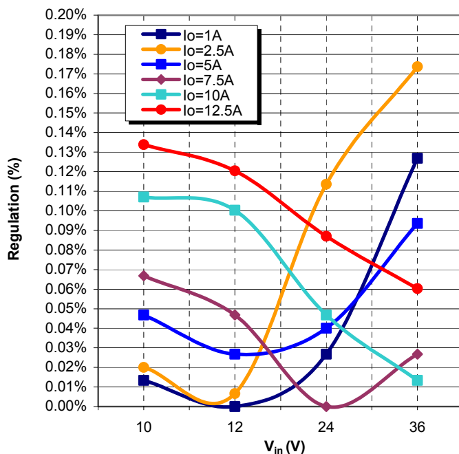
Graph 10: LV12S12-150 Line Regulation ( \pm RS Pins Open)
