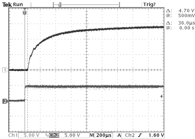
Photo 1: Remote Turn On Vin=24V, Iout = 1.25A
