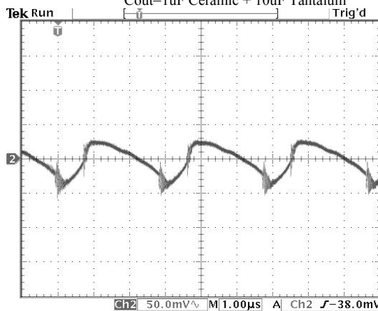
Photo 8: Transient Response Min Load to Max Load Vin=24V, Iout = 1.25 to 12.5A Cout=1uF Ceramic + 10uF Tantalum
