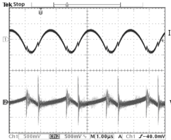
Photo 10: Output Voltage Ripple (20 MHz BW) Vin=24V, Iout=12.5A Cout=1uF Ceramic + 10uF Tantalum
