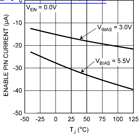
Enable Pull-Down Current ( I_{EN} ) vs Temperature 查询"LP38852S-ADJ"供应商
