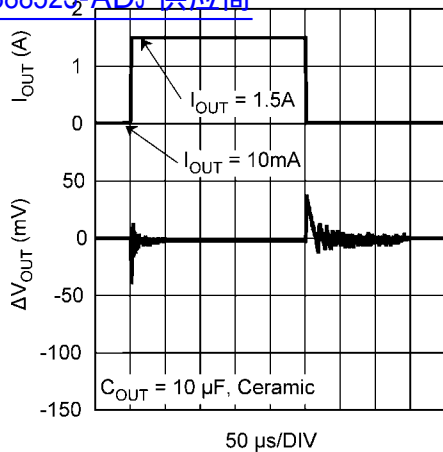
Load Transient Response, C_{OUT} = 10\ \mu\text{F} Ceramic 查询"LP38852S-ADJ"供应商
