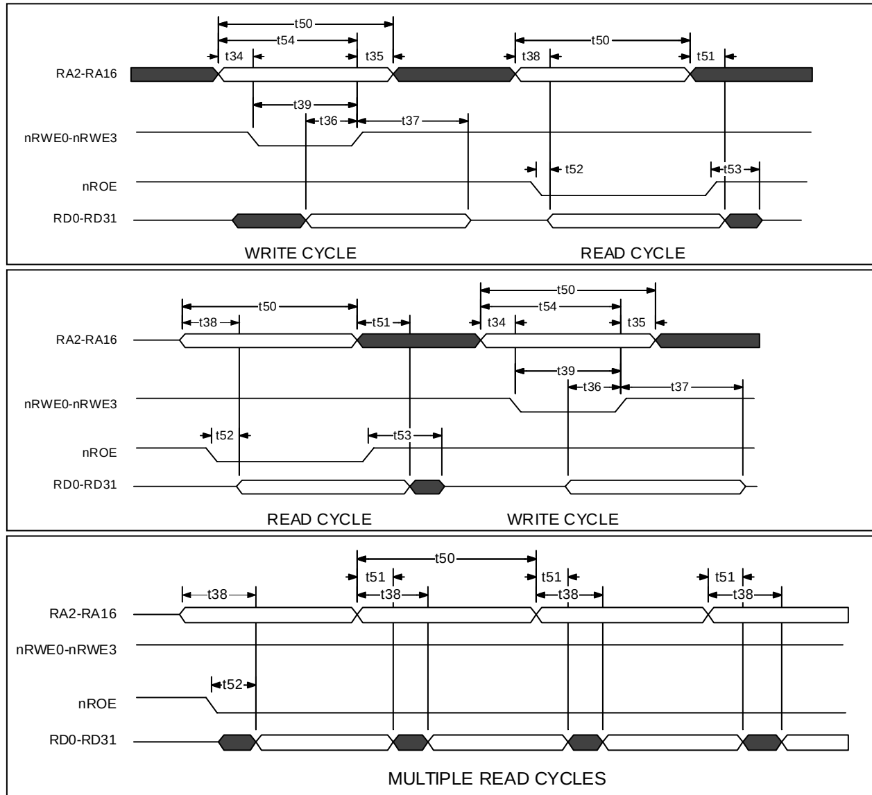
Figure 9.9 - SRAM Interface
