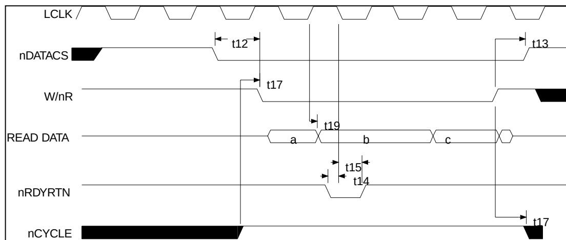
Figure 9.5 - Burst Read Cycles - nVLBUS=1
