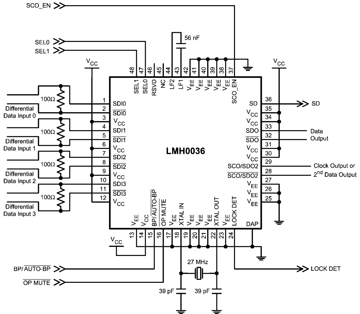
FIGURE 4. Application Circuit
