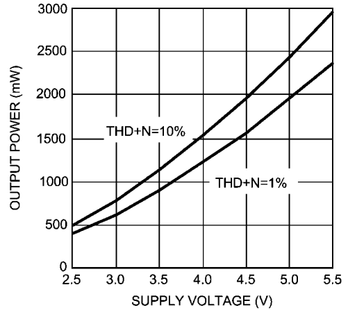
Output Power vs Supply Voltage R_L = 4\Omega, f = 1kHz
