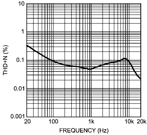
THD+N vs Frequency V_{DD} = 3.6V, R_L = 8\Omega, P_O = 250mW/channel
