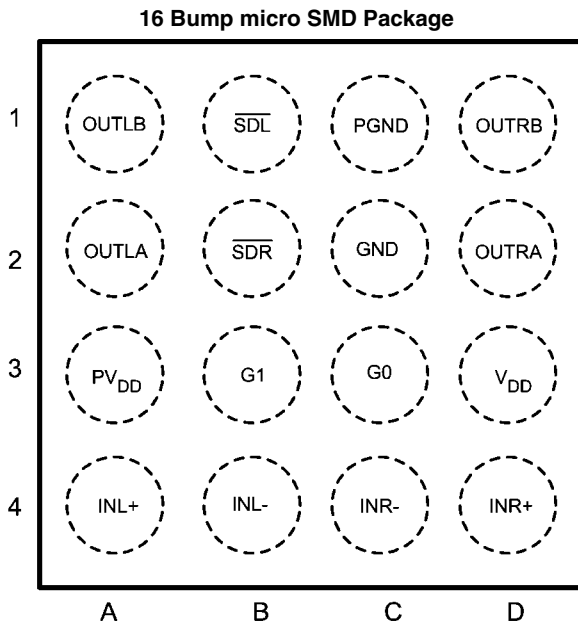
Top View Order Number LM48411TL See NS Package Number TLA16ACA
