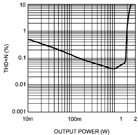
THD+N vs Output Power V_{DD} = 3.6V, R_L = 4\Omega, A_V = 24dB
