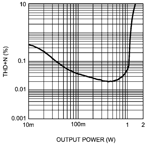
THD+N vs Output Power V_{DD} = 5V, R_L = 8\Omega, A_V = 6dB
