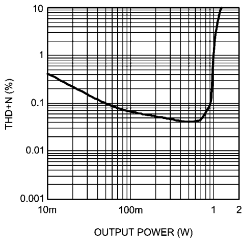
THD+N vs Output Power V_{DD} = 3.6V, R_L = 4\Omega, A_V = 6dB
