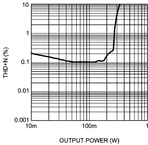
THD+N vs Output Power V_{DD} = 2.5V, R_L = 8\Omega, A_V = 6dB
