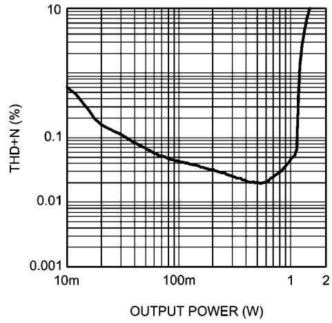
THD+N vs Output Power V_{DD} = 5V, R_L = 8\Omega, A_V = 24dB
