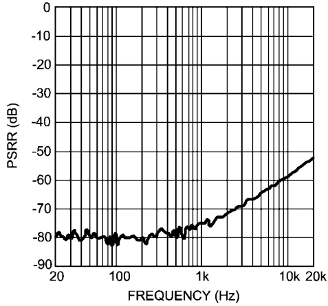
PSRR vs Frequency V_{DD} = 3.6V, R_L = 8\Omega
