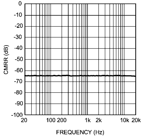
CMRR vs Frequency V_{DD} = 3.6V, R_L = 8\Omega
