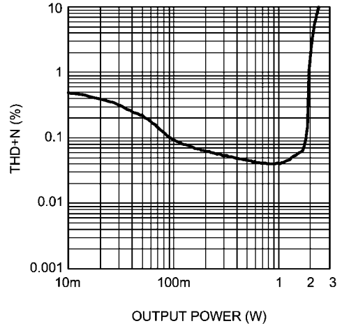
THD+N vs Output Power V_{DD} = 5.0V, R_L = 4\Omega, A_V = 24dB
