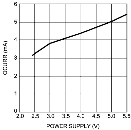
Quiescent Current vs Power Supply R_L = \infty
