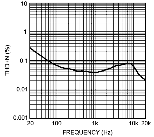
THD+N vs Frequency V_{DD} = 5.0V, R_L = 4\Omega, P_O = 375mW/channel
