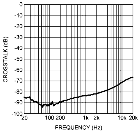
Crosstalk vs Frequency V_{DD} = 3.6V, R_L = 8\Omega
