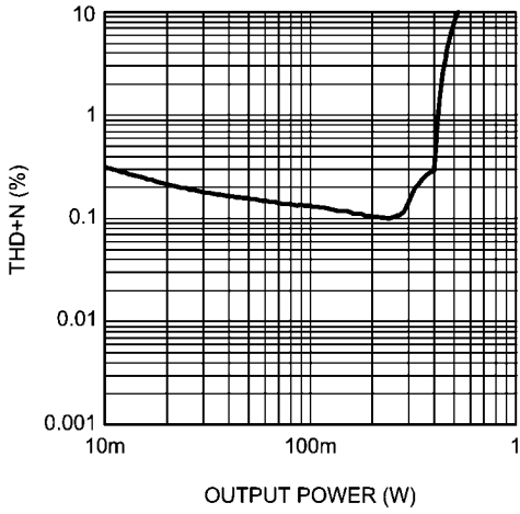
THD+N vs Output Power V_{DD} = 2.5V, R_L = 4\Omega, A_V = 6dB
