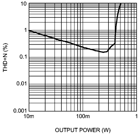
THD+N vs Output Power V_{DD} = 2.5V, R_L = 4\Omega, A_V = 24dB
