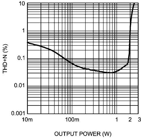
THD+N vs Output Power V_{DD} = 5.0V, R_L = 4\Omega, A_V = 6dB
