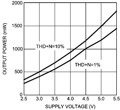
Output Power vs Supply Voltage 查询"LM48411"供应商 R_L = 8\Omega, f = 1kHz
