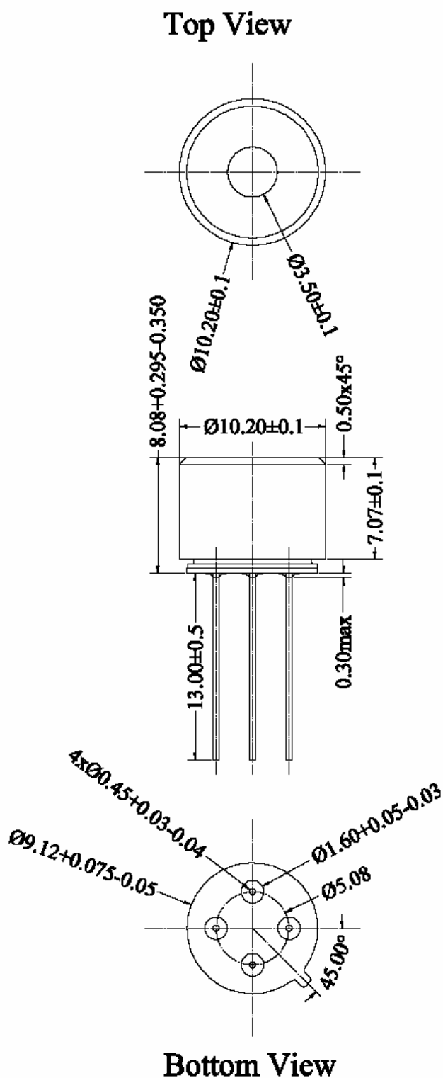
Figure 29: MLX90614XXC package
