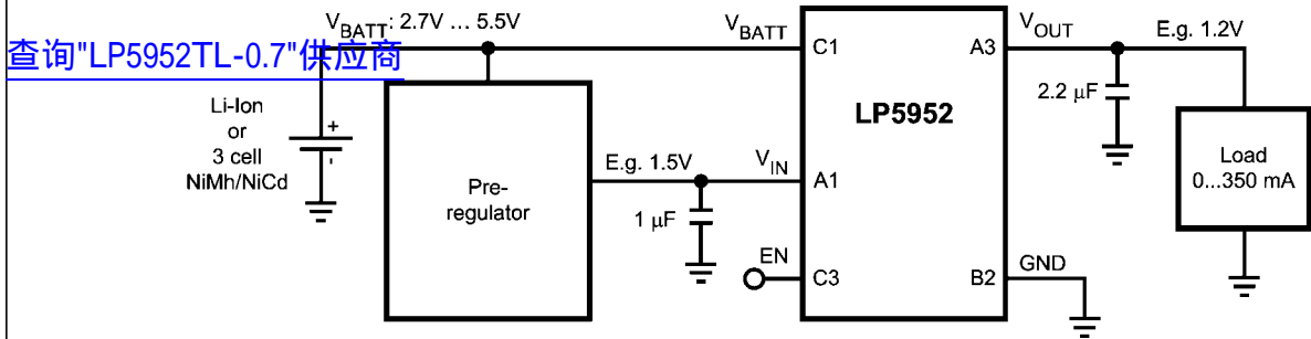
FIGURE 2: Typical Application Circuit
