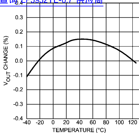
Output Voltage Change vs Temperature 查询"LP5952TL-0.7"供应商
