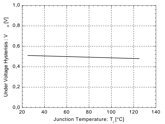
Under Voltage Hysteresis vs. Junction Temperature
