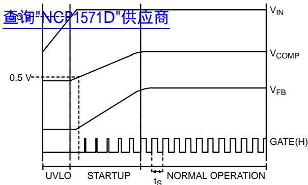
Figure 22. Idealized Waveforms
