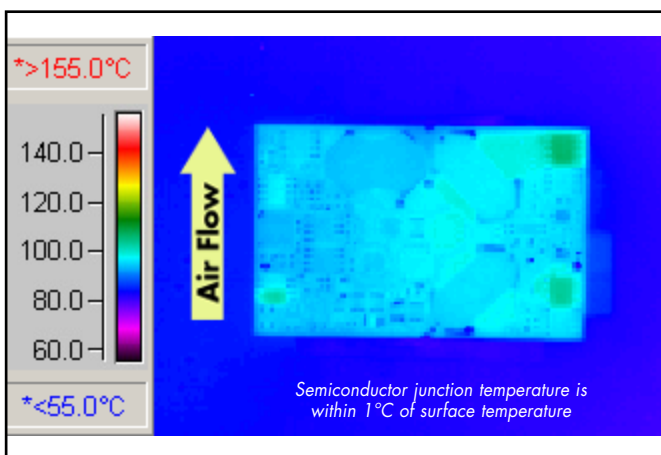
Figure 18: Thermal plot of converter at 12 amp load on 1.225V output and 2 amp load on 2.45V output with 85^{\circ}\text{C} air flowing at 200 LFM. Air flow across the converter is from pin 3 to pin 1 (nominal input voltage).
