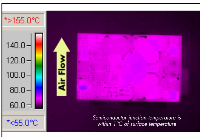
Figure 14: Thermal plot of converter at 8 amp load on 2.45V output and no load on 1.225V output with 55^{\circ}\text{C} air flowing at 200 LFM. Air flow across the converter is from pin 3 to pin 1 (nominal input voltage)
