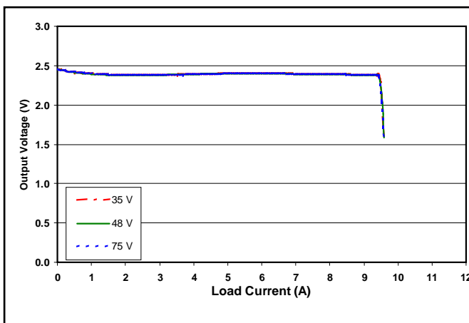
Figure 28: Output voltage vs. load current showing typical current limit curves and converter shutdown points for the 2.45V output. 1.225V load is at 0A.
