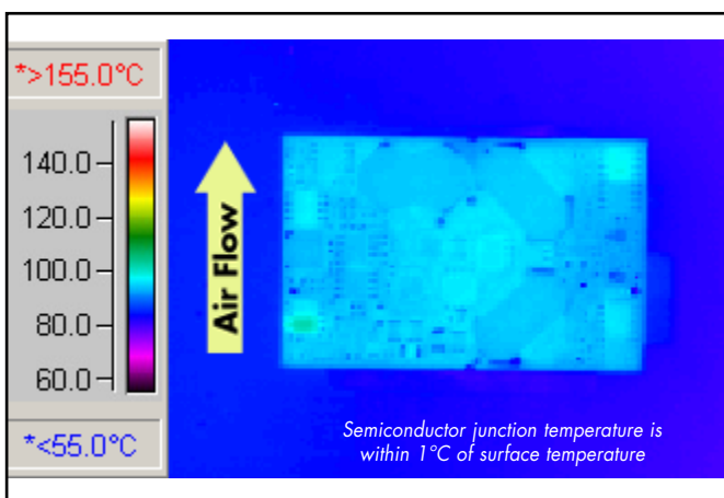
Figure 16: Thermal plot of converter at 8 amp load on 1.225V output and 4 amp load on 2.45V output with 85^{\circ}\text{C} air flowing at 200 LFM. Air flow across the converter is from pin 3 to pin 1 (nominal input voltage)
