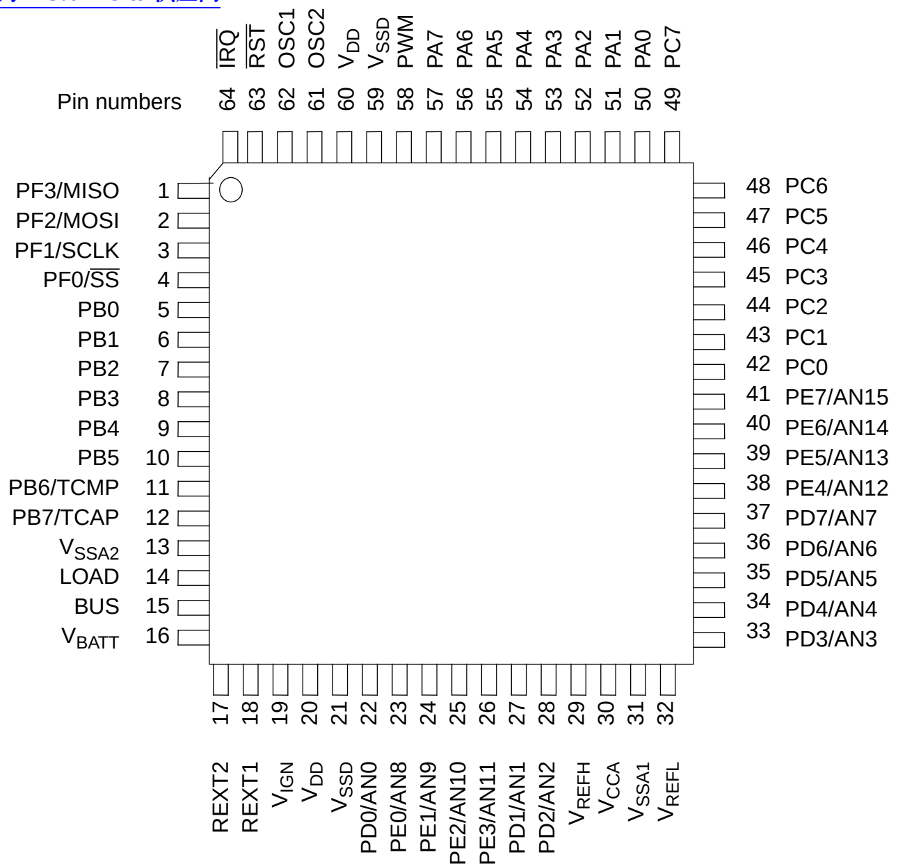
Figure 1-3: MC68HC05V7 Pin Assignments (64-pin QFP)
