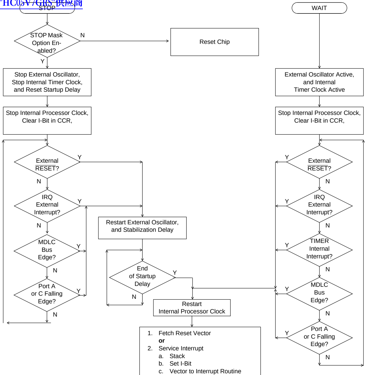
Figure 8-2: STOP/WAIT Flowcharts
