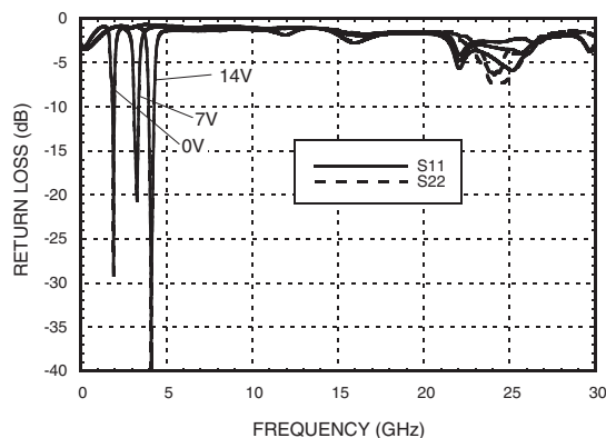
Broadband Return Loss vs. Control Voltages, V_{fctl} = V_{bwctl}
