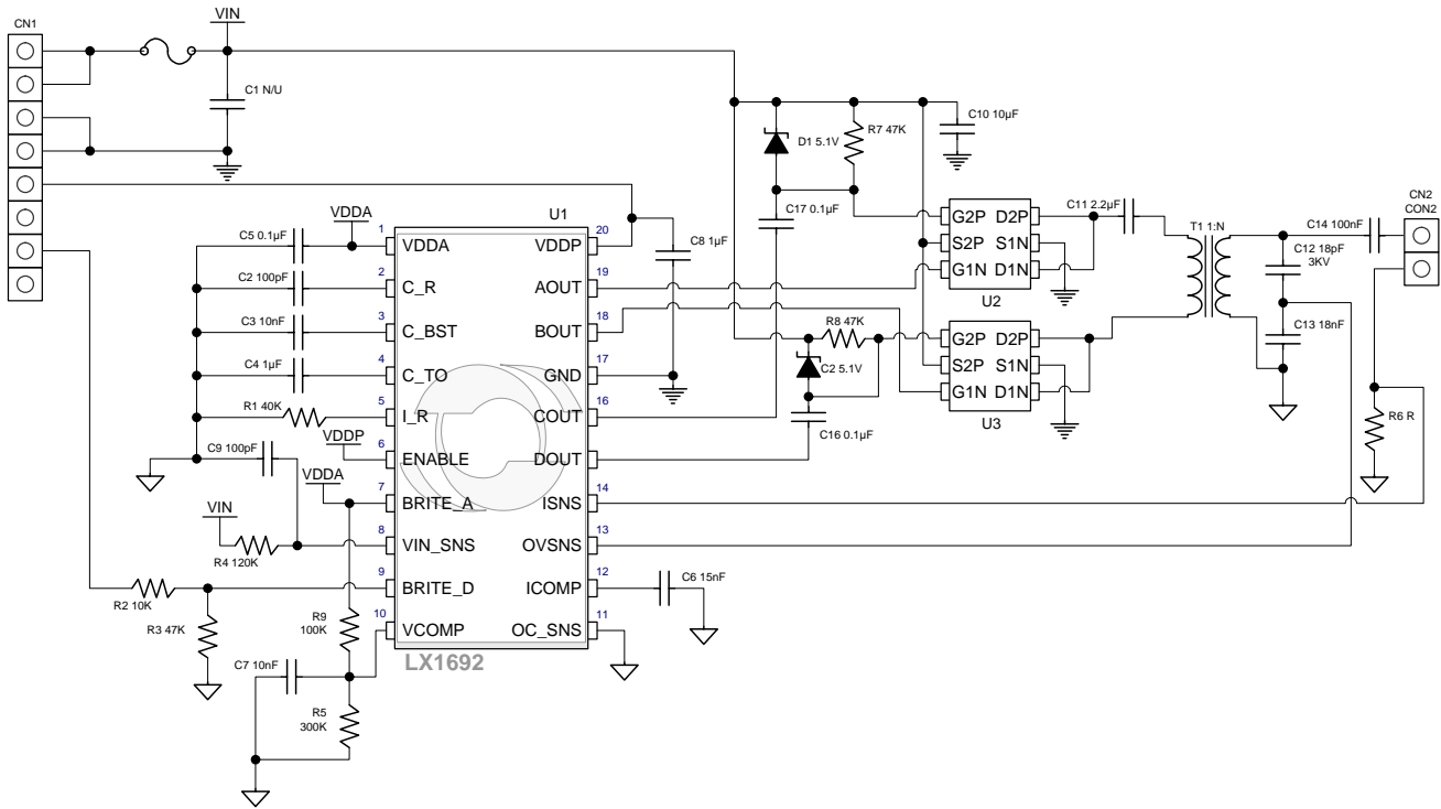
Figure 3 – Schematic
