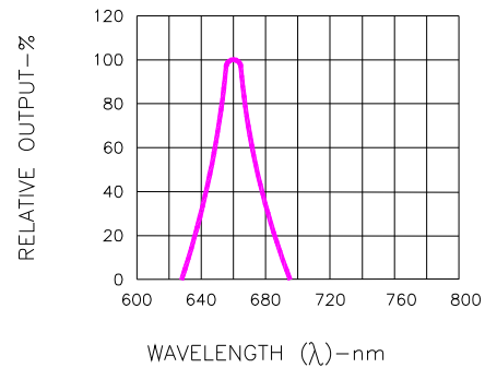
Fig.2 SPECTRAL RESPONSE
