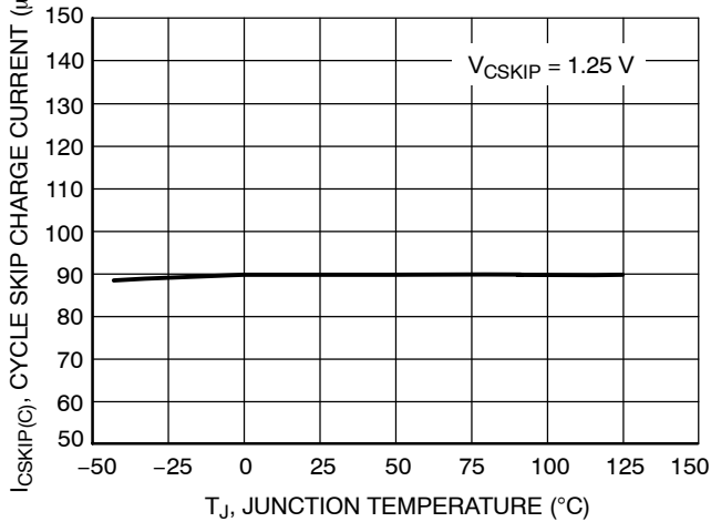
Figure 18. Cycle Skip Charge Current vs. Junction Temperature
