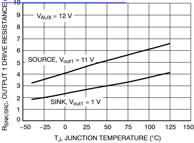
Figure 30. Output 1 Drive Resistance vs. Junction Temperature
