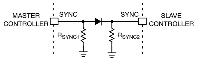
Figure 50. Master-Slave Configuration
