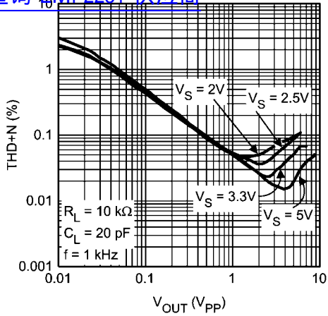
THD+N vs. Amplitude 查询"LMP2231"供应商
