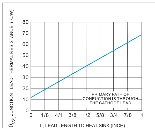
FIGURE 10. TYPICAL THERMAL RESISTANCE
