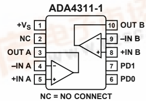
Figure 1. Thermally Enhanced, 10-Lead MINI_SO_EP
