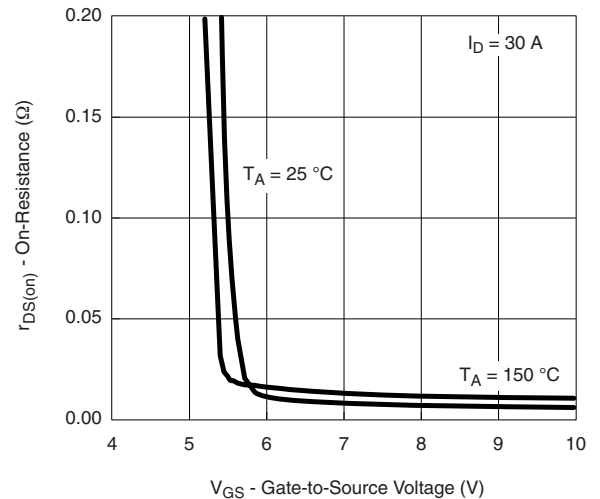
On-Resistance vs. Gate-to-Source Voltage vs. Temperature
