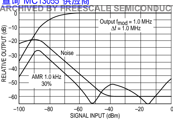
Figure 3. Overall Gain, Noise, AM Rejection
