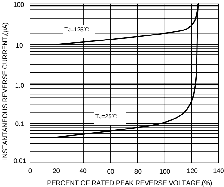
FIG.5-TYPICAL REVERSE CHARACTERISTICS
